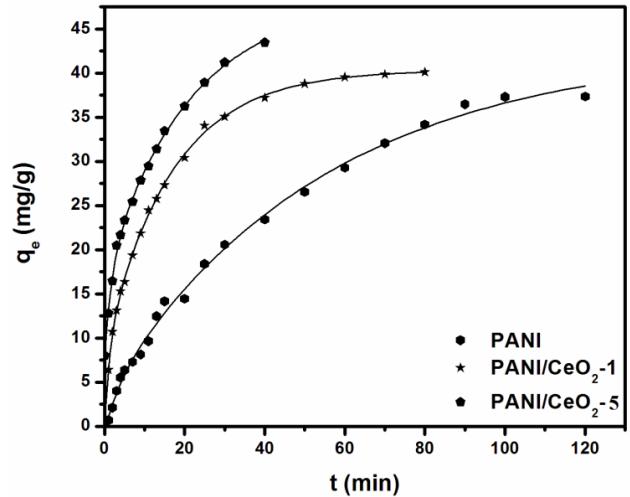
Fig. 8 The variation in adsorption capacity with adsorption time for Remazol Red RB- 133 dye onto PANI and PANI/CeO 2 nanocomposites (dye concentration is 50 mg L -1 , adsorbent dosage = 0.1 g L -1 , pH = 6.5).
